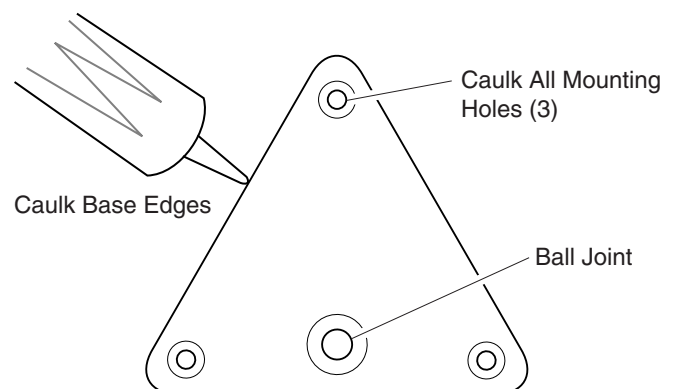
Three Mounting Holes for Solar Panel Base
