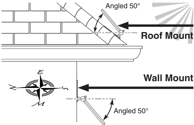
Mounted Solar Panel
